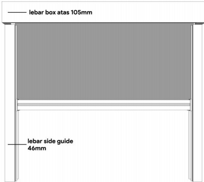
Cover box With Frame
